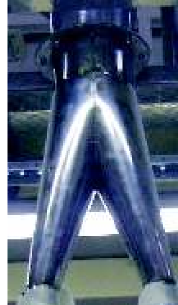
Food industry standard stainless steel hoppers filling points and breeches pieces.
